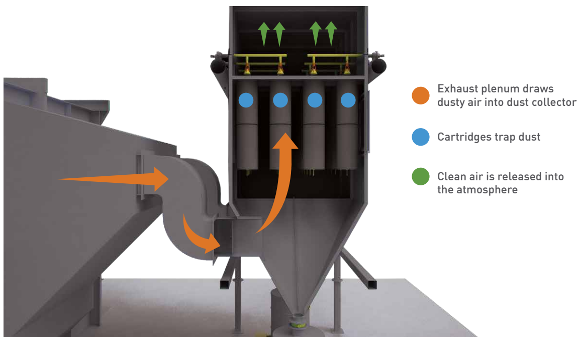
DIAGRAM SHOWS THE PATH OF THE AIRFLOW
