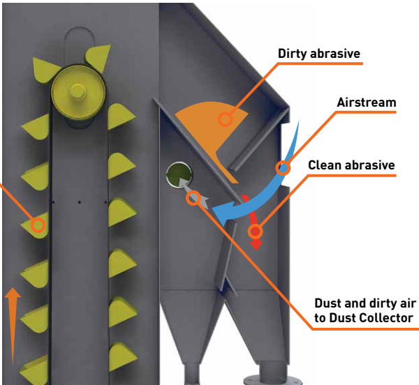
Abrasive is conveyed up by a bucket elevator
